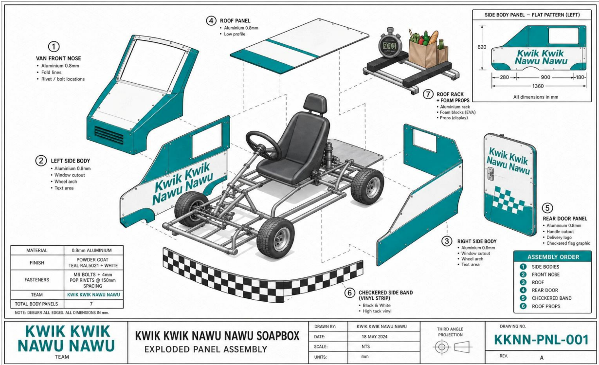
Image 5 — Detailed View (Exploded View)
